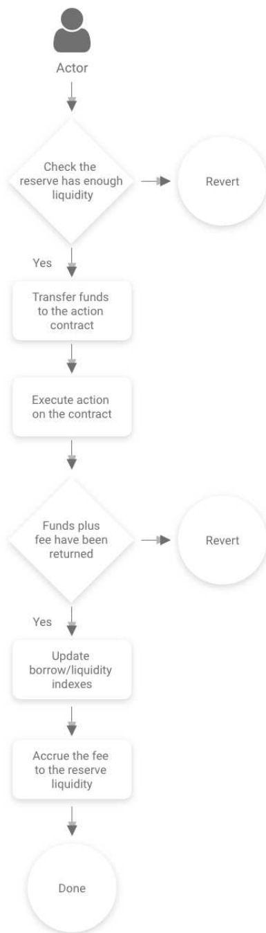
Figure 12: Flash Loan
